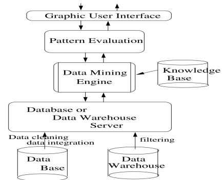
Figure 1.5: Architecture of a typical data mining system.
